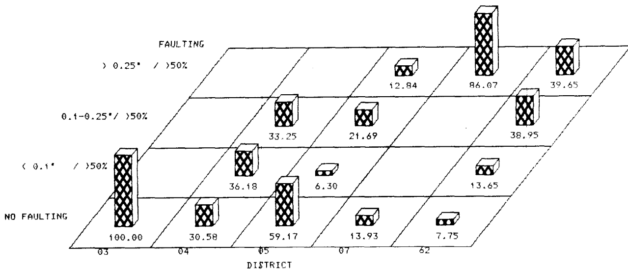
Figure 5-7 Percent of Miles of JCP in Districts by Magnitude of Faulting
