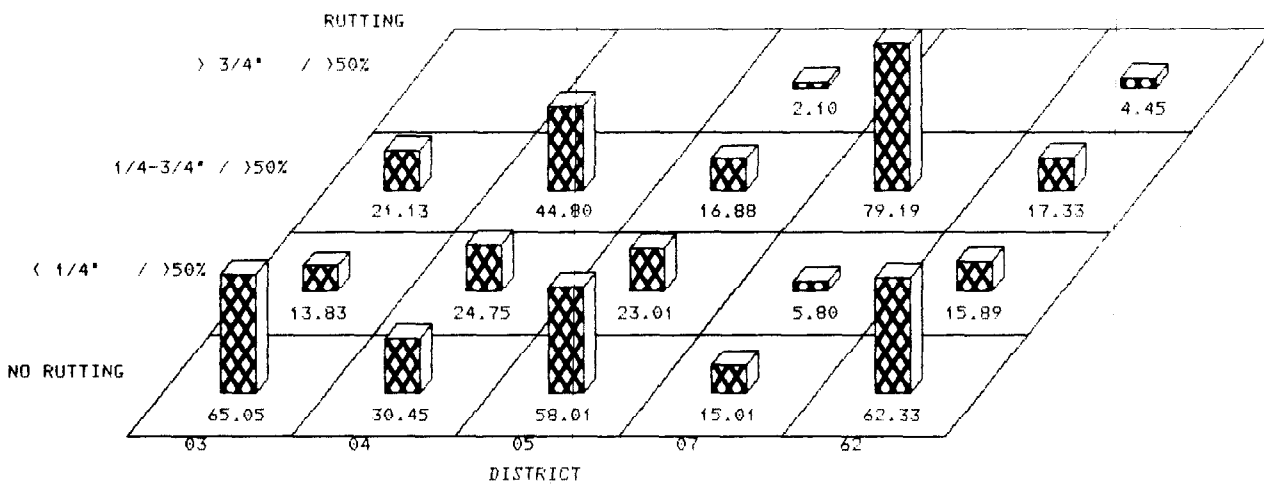
Figure 5-6 Percent of Miles of Hot Mix Pavement in Districts by Magnitude of Rutting
