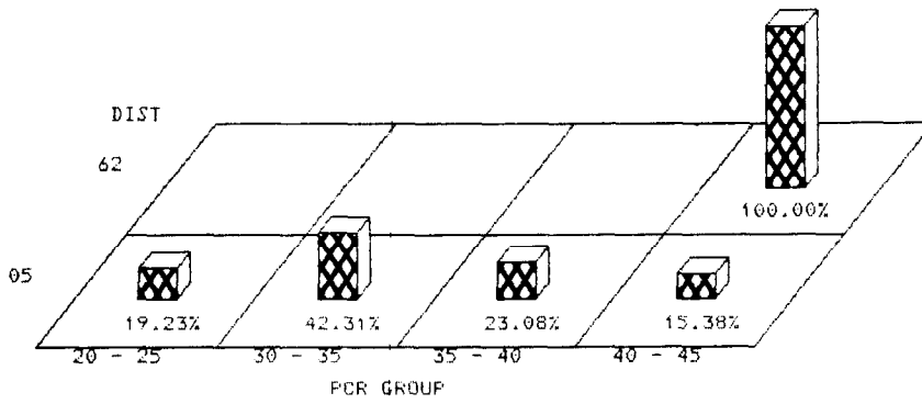
Figure 5-5 Percent of Miles of Continuously Reinforced Concrete Pavements by Districts & PCR Index
