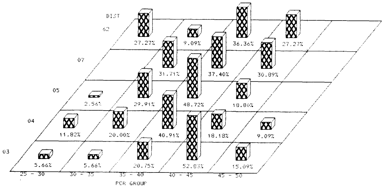
Figure 5-4 Percent of Miles of Composite Pavements by District & PCR Index
